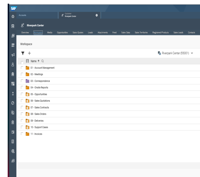
SAP C/4HANA(C4C)
