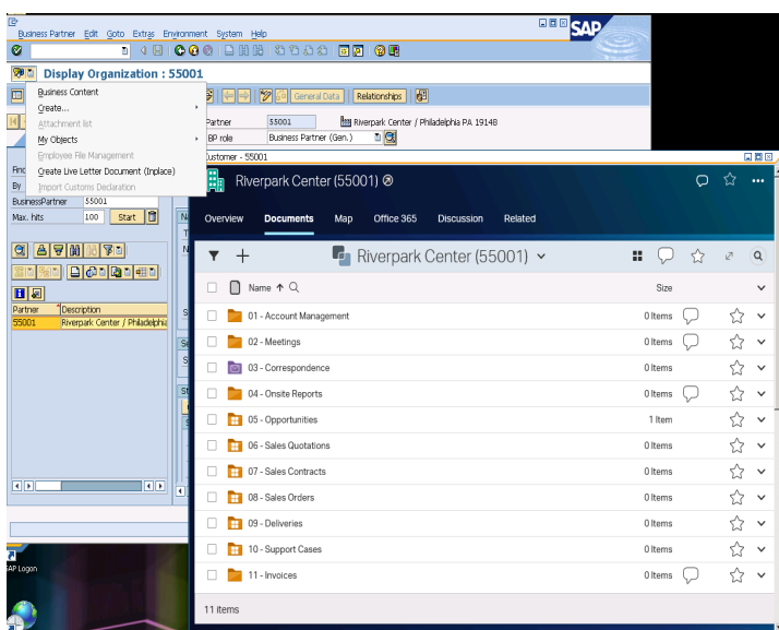
SAP Netweaver
